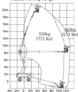
AR20JE Working Range
