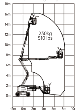
AR14J Working Range
